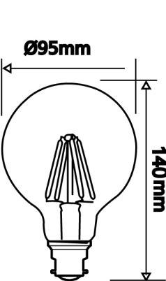
G959-12 LINE DRAWING
