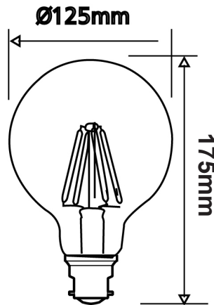
G1259-12 LINE DRAWING
